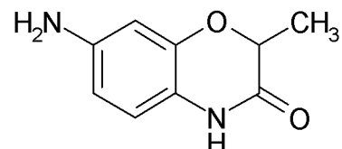
7-amino-2-methyl-2H-1,4-benzoxazin-3(4H)-one KLD-244
