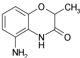
5-amino-2-methyl-2H-1,4-benzoxazin-3(4H)-one KLD-322
