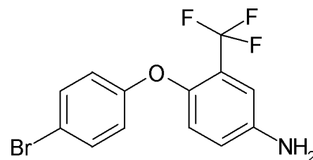
4-(4-bromophenoxy)-3-(trifluoromethyl)aniline KTD-310
