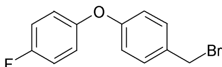
1-(bromomethyl)-4-(4-fluorophenoxy)benzene KTD-015
