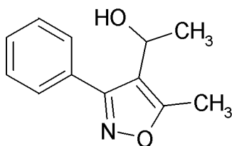
1-(5-methyl-3-phenylisoxazol-4-yl)ethanol KTD-350
