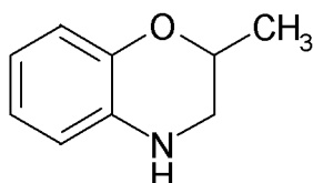
2-methyl-3,4-dihydro-2H-1,4-benzoxazine KLD-147
